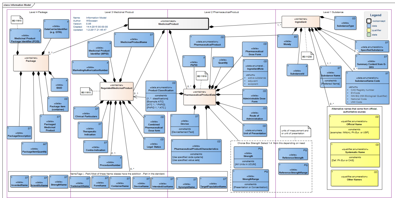
Figure 1. Detailed Clinical Model in UML for a Medicinal Product (draft 0.85).
